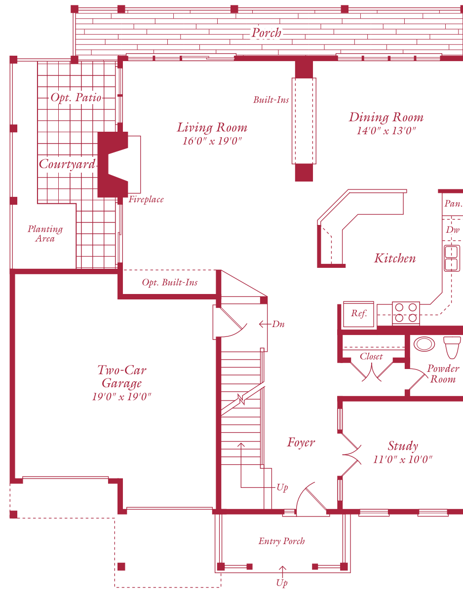
Main Level
